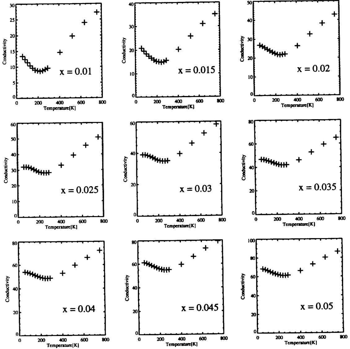
Figure 3.1b Conductivity as a function of temperature for r=1.5 .
